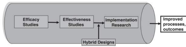
FIGURE 1. Research pipeline.
